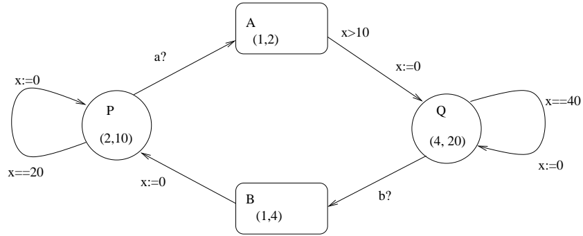
Figure 5. Timed Automaton with Periodic and Sporadic Tasks.
